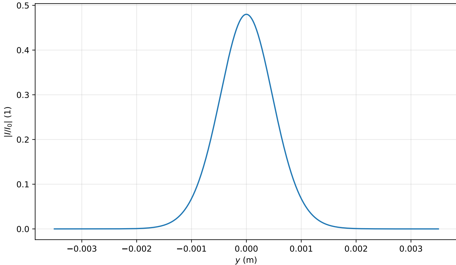
Intensity profile I(x = 0, y, z = 2.707)/I_0 , P_{in}=0.3P_{cr} , artificial time
